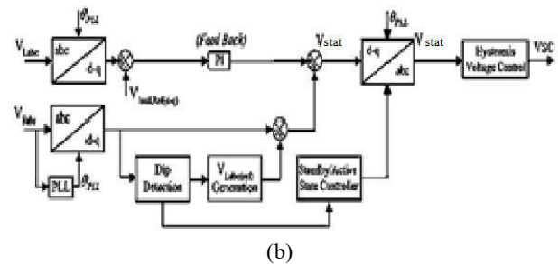
Fig.5.(a)d-q Transformation (b) Control structure of STATCOM
