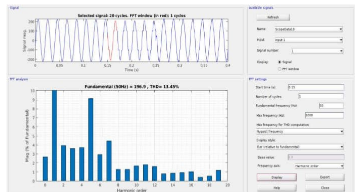
Fig.8.Totalharmonicdistortionofthecompensatedvoltage
