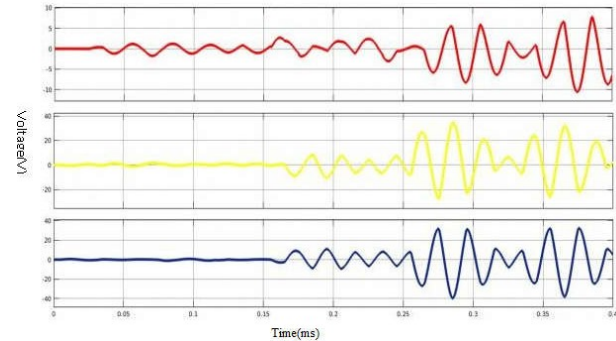
Fig.8.Compensated Load voltage from PV-
