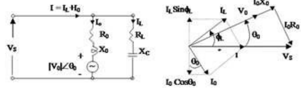
Fig.2. Inductive mode of operation
