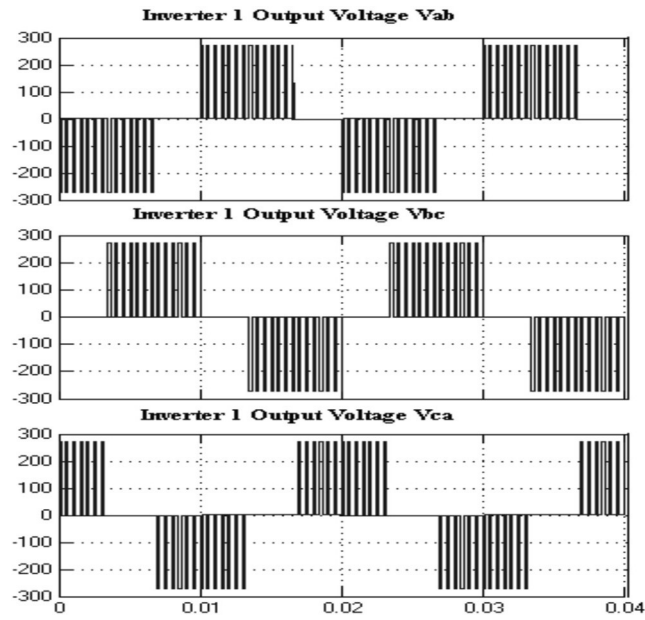
Figure10a:Inverter1outputvoltageVab,Vbc,VcaforModulationIndex=0.9
