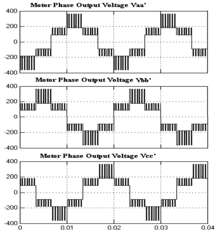
Figure10cMotorPhasevoltageVaa',Vbb',Vcc'forModulationIndex=0.9.
