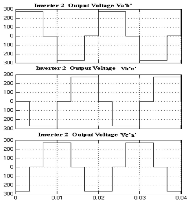
Figure10b:Inverter2outputvoltageVa'b',Vb'c',Vc'a'forModulationIndex=0.9.
