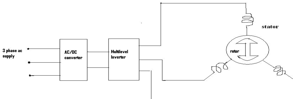
Figure2MultilevelInverter(MLI)forInductionMotorDrive
