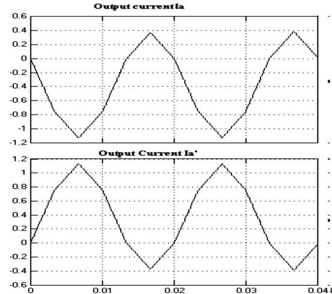
Figure10dOutputCurrentIaandIa'forModulationIndex=0.9.
