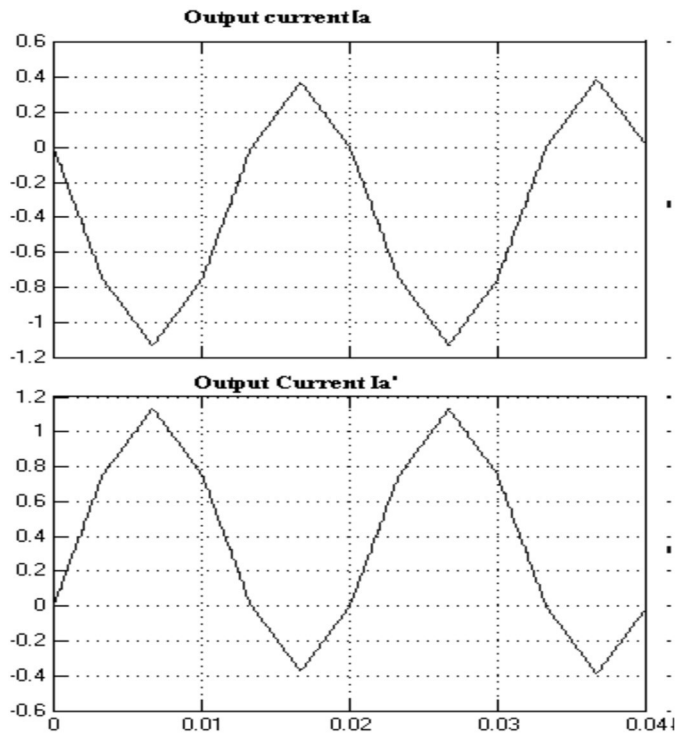
Figure11d:OutputCurrentIaandIa'forModulation Index=0.9.
