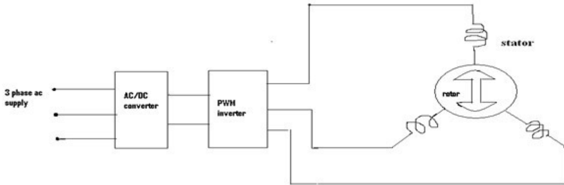
Figure1 PWMInverterforInductionMotorDrive
