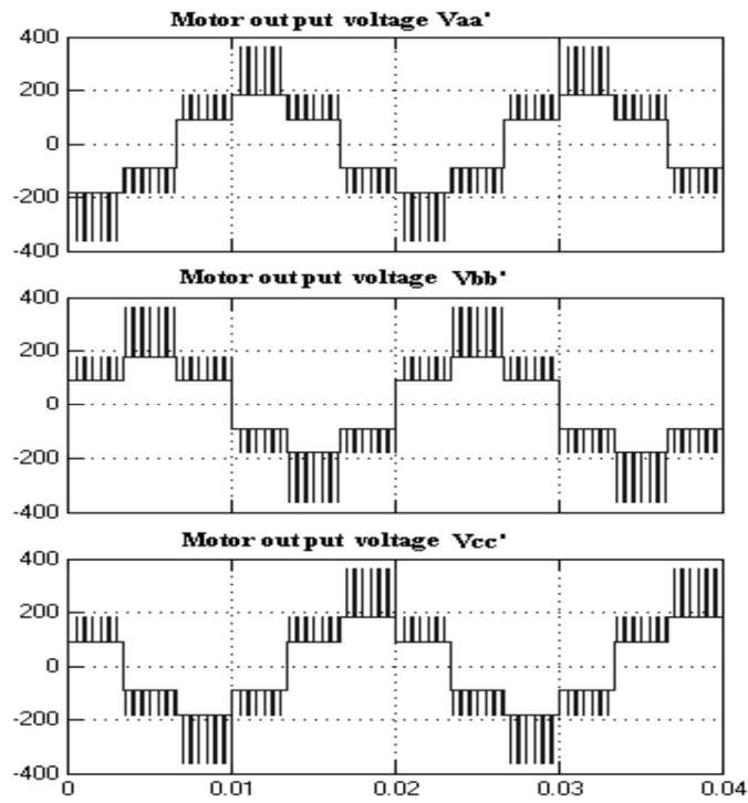
Figure11cMotorPhasevoltageVaa',Vbb',Vcc'forModulationIndex=0.9.
