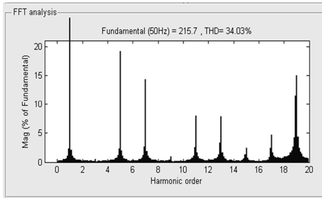
Figure12Spectrumwaveformforthreelleveloutput
