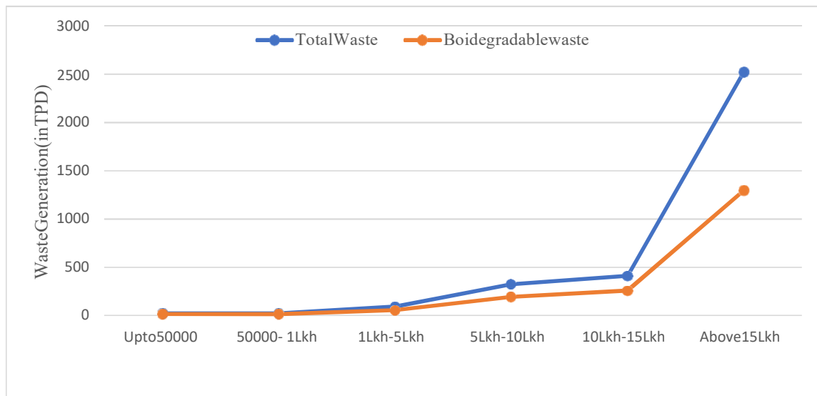
Figure2:TotalgeneratedMSWtoBiodegradablewaste
