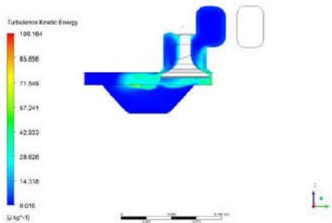
Turbulent kinetic energy at 60° crank angle
