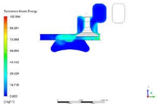
Turbulent kinetic energy at 60° crank angle
