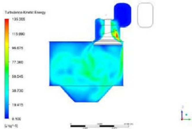
Turbulent kinetic energy at 160° crank angle
