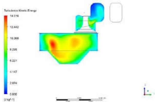
Turbulent kinetic energy at 240° crank
