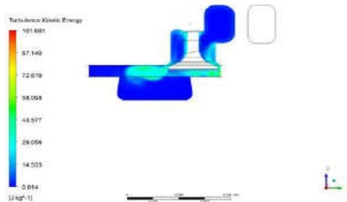
Turbulent kinetic energy at 60° crank angle
