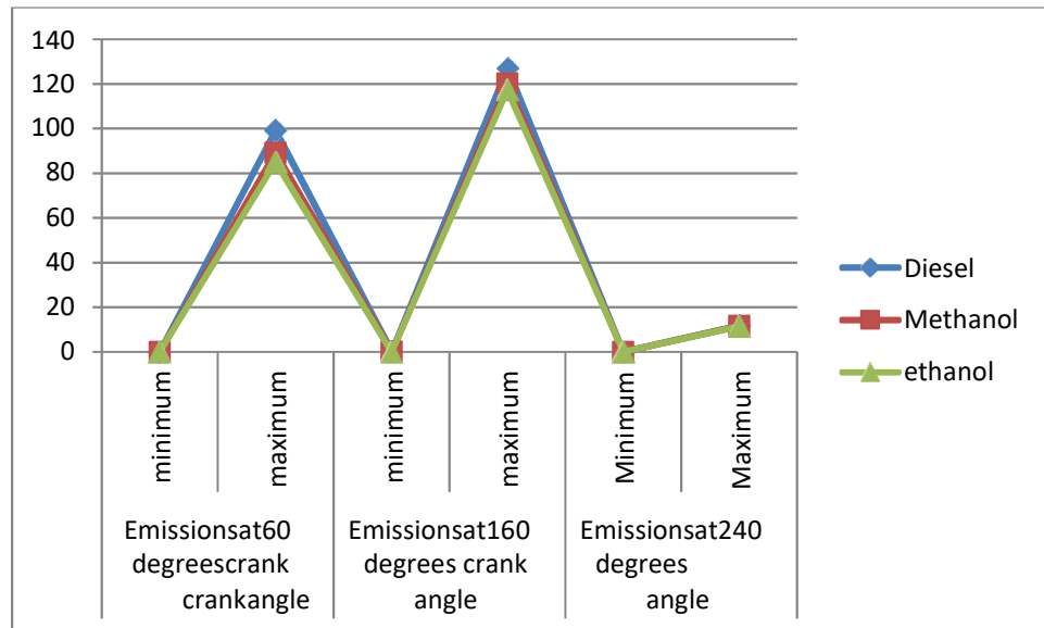
Variations in CO emissions released at different points due to use of different fuels at different crank angles
