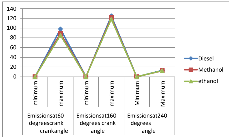
Variations in CO 2 emissions released at different points due to use of different fuels at different crank angles
