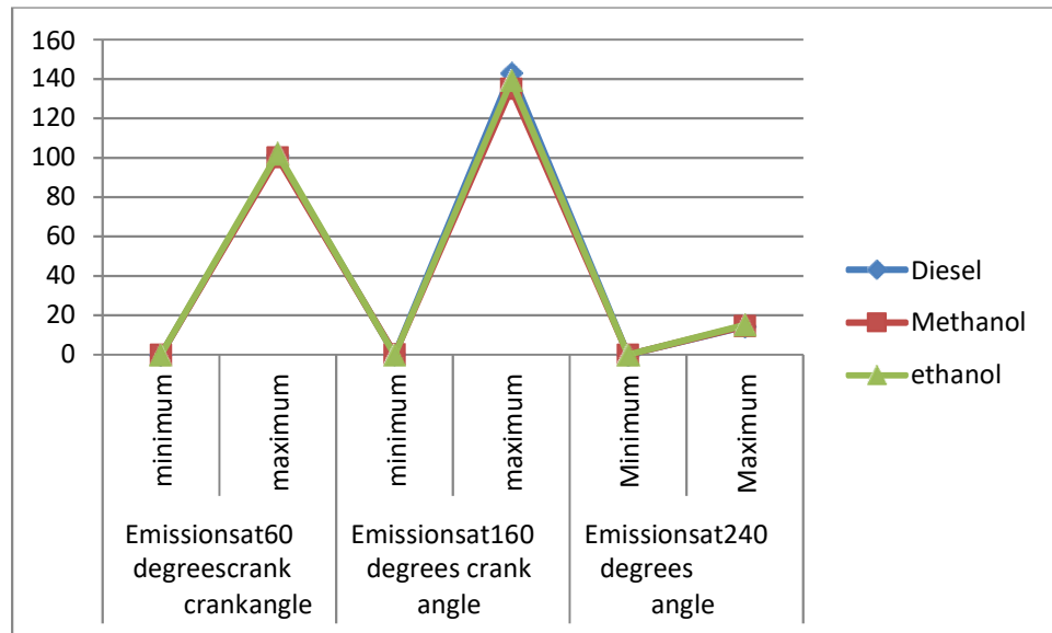
Variations in NOx emissions released at different points due to use of different fuels at different crank angles
