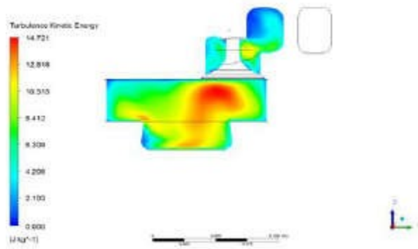
Turbulent kinetic energy at 240° crank angle
