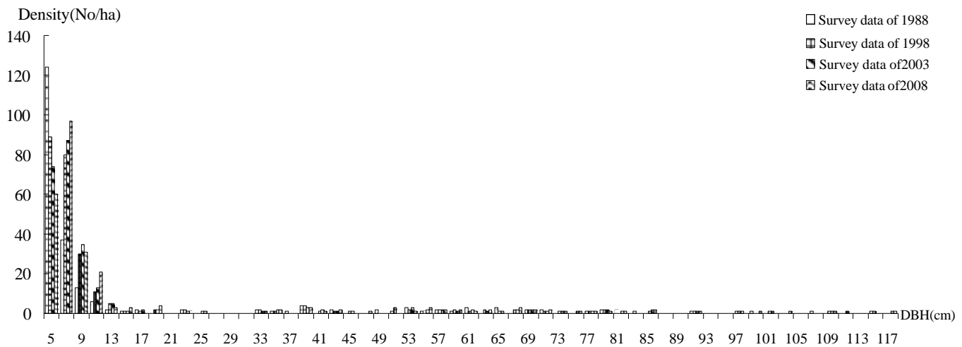
Figure 5. Survey data of changes in DBH distribution of broad-leaved trees
