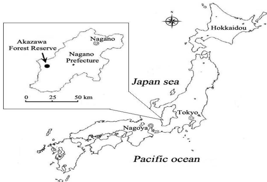
Figure.1 The location of Akazawa Forest Reserve
