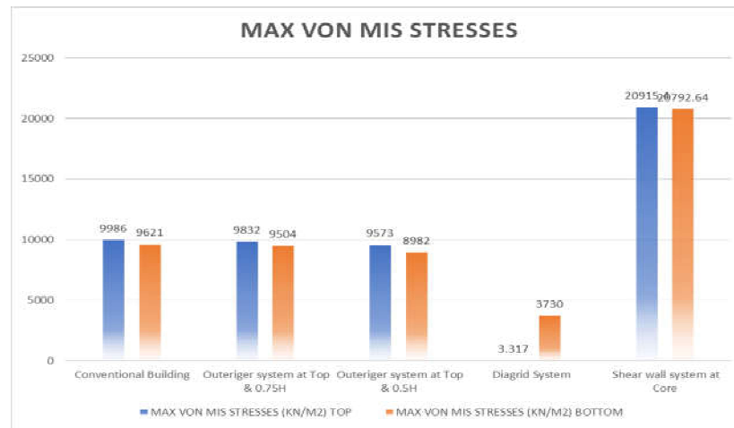
Graph6MaxVonMisstresssinSlab
