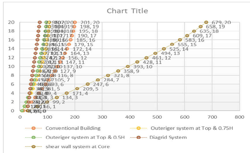
Graph2StoreyShearindifferentloadresistingsystem
