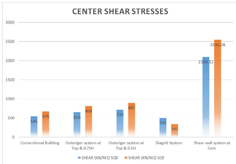
Graph4CenterShearStressesVsDifferenttypesofBuilding
