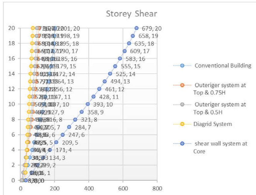
Graph3StoreyDriftindifferentloadresistingsystem
