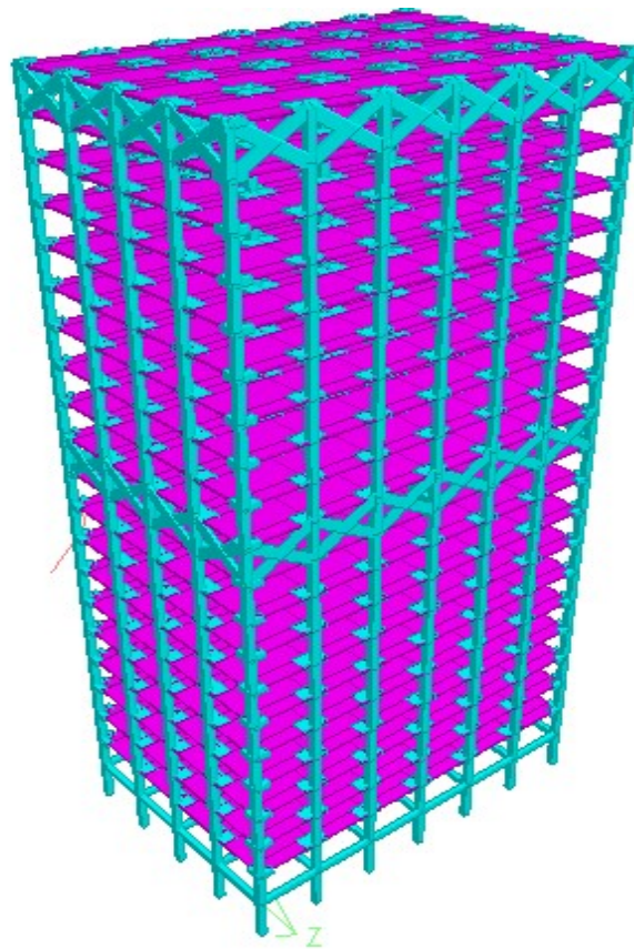
Fig-3:steeloutriggersystemBuilding
