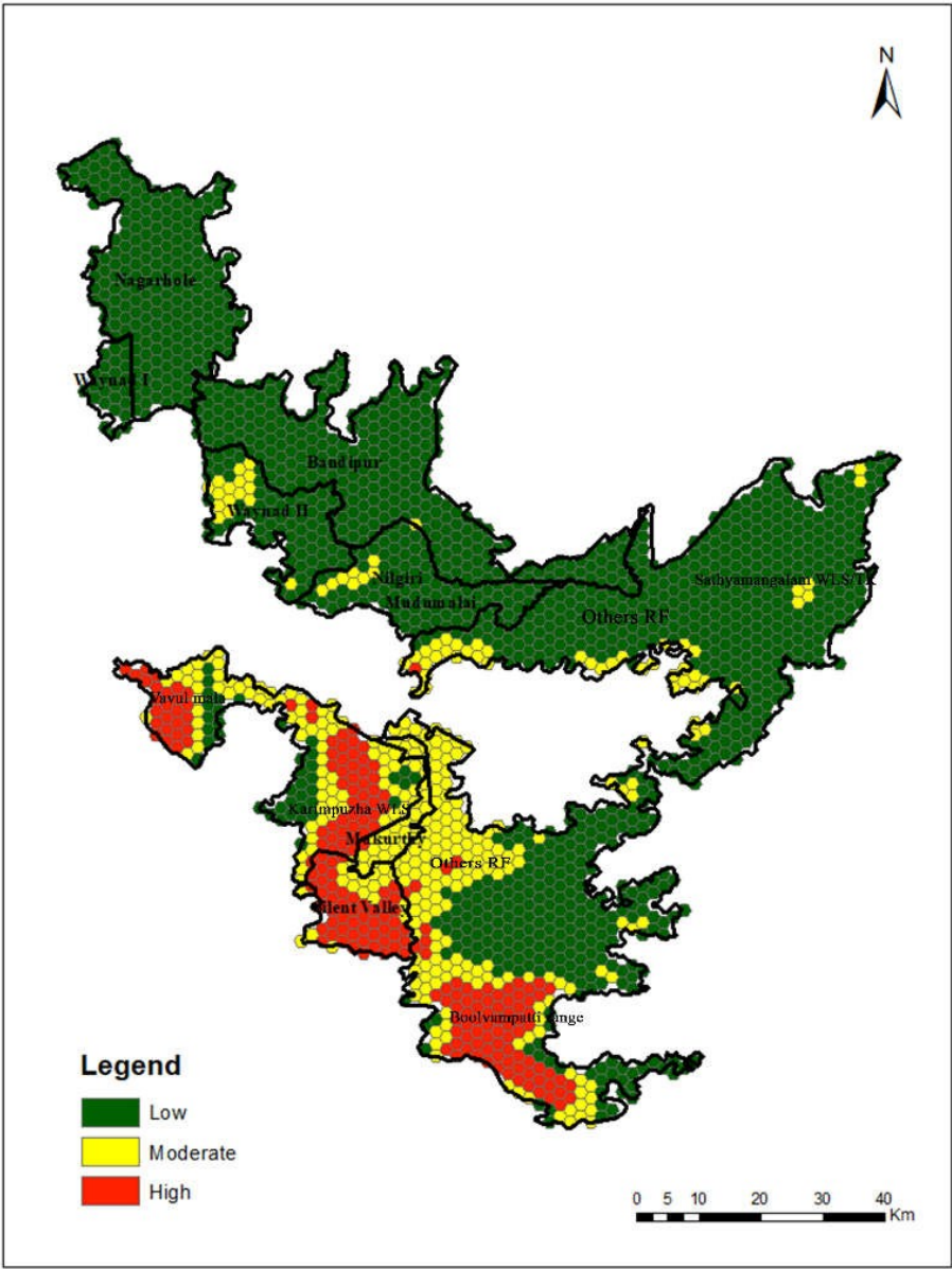
Fig.3 Speciesrichness( SR_{end} )ofendemicvascularplantinNilgiriBiosphereReserve
