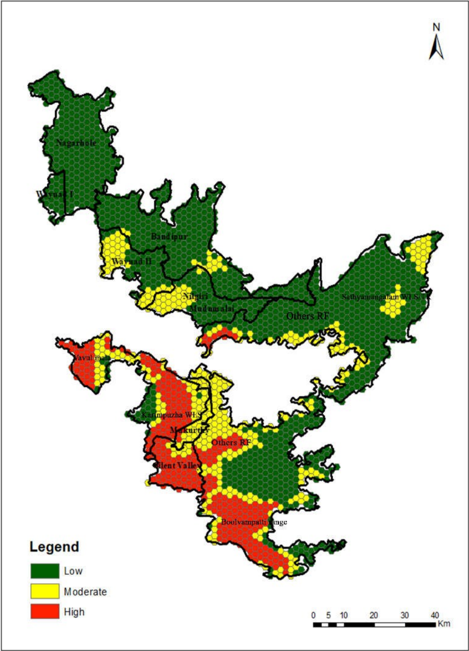
Fig.5 WeightedEndemism(WE end )inNilgiriBiosphereReserve
