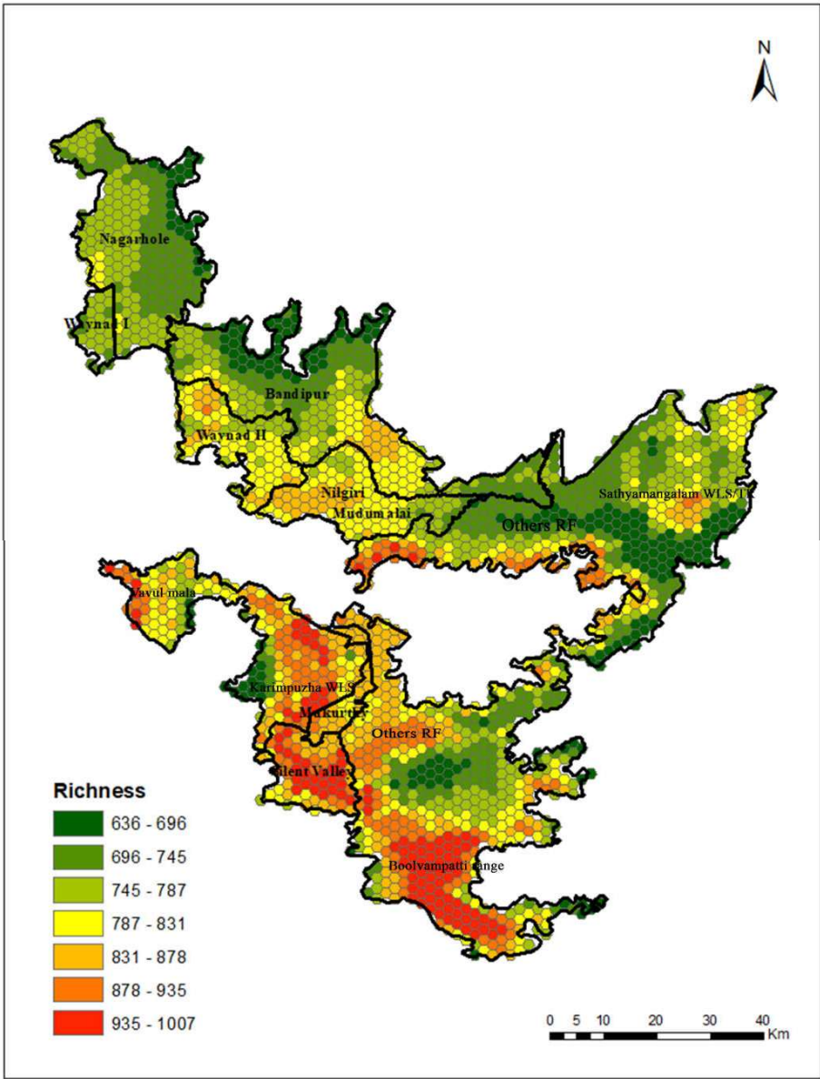
Fig. 2 Biodiversityspeciesrichness( SR_{biodiv} )inNilgiriBiosphereReserve(NBR)
