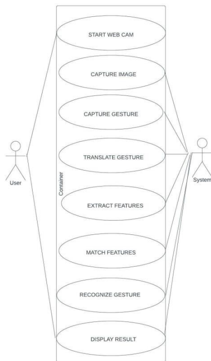
Fig3: Usecase diagram
