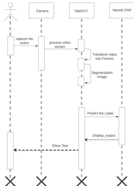
Fig1: Sequenced diagram
