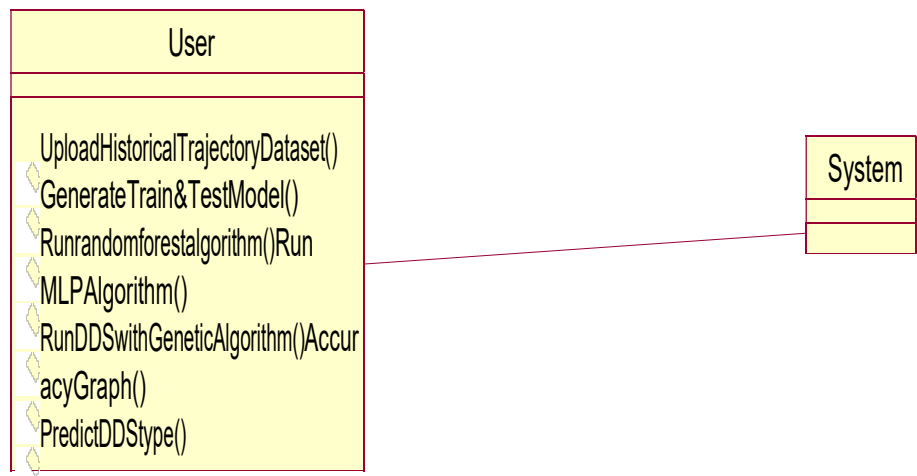
Fig4.3:ClassDiagram
