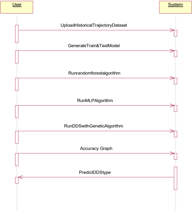
Fig4.4:SequenceDiagram
