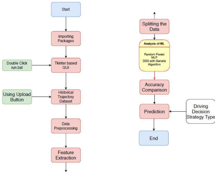
Fig:Flowchart
