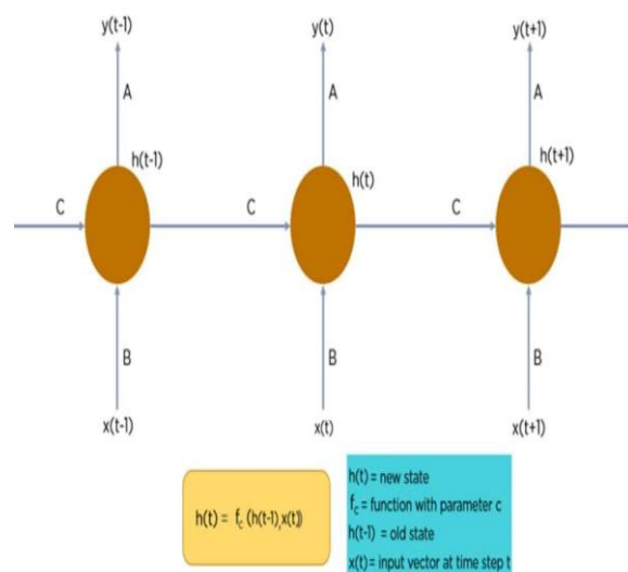
Fig 4 Functions of RNN
