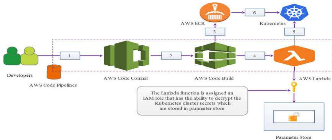
Figure3:Amazonweb services
