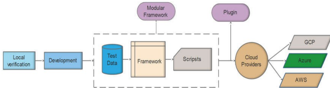
Figure5:proposedFrameworkofContinuousTestingModularFramework
