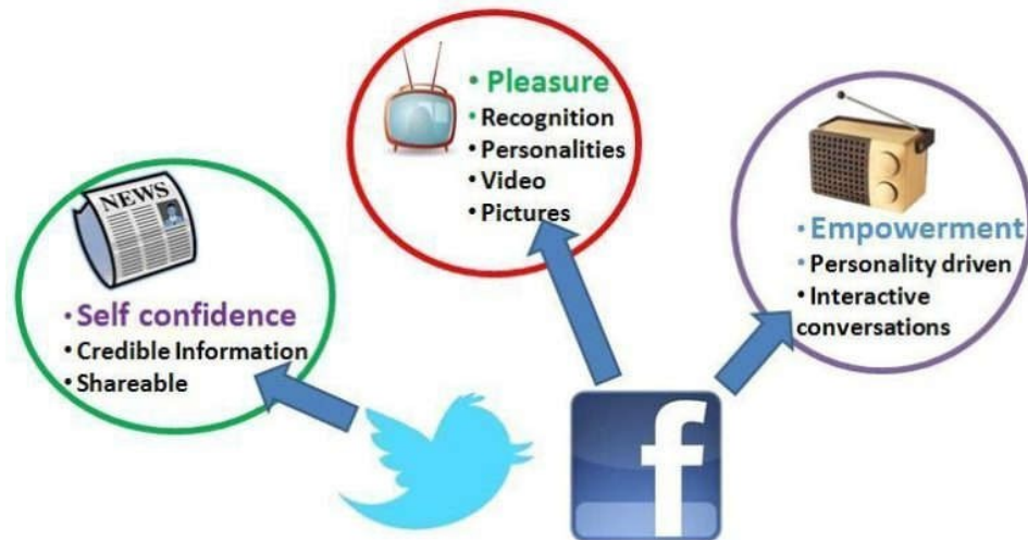
Fig1.:Uses&GratificationSocialMediaModelSo
