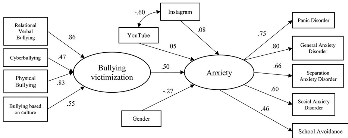
Fig2:Structuralequationmodelbetweenvariables.
