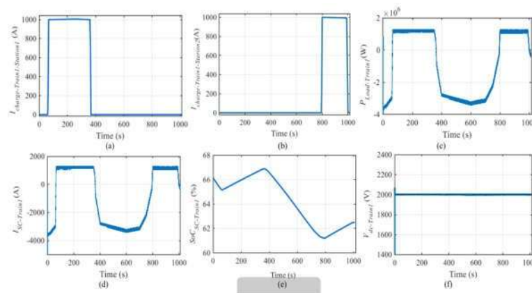
FIGURE8. Simulation test of train 1.(a)Charge current to train 1 from station 1.(b)Charge current to train 1 from station 2.(c)Load power of train 1.(d)SC current of train 1.(e)SoC of SC of train 1.(f)DC bus voltage of train 1.
