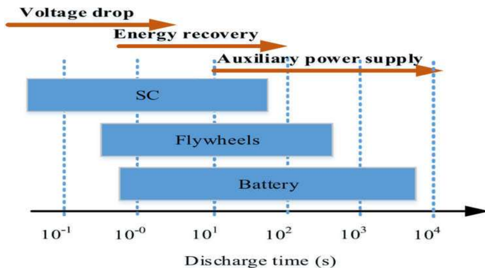
FIGURE3. Classification of ES technologies [22].
