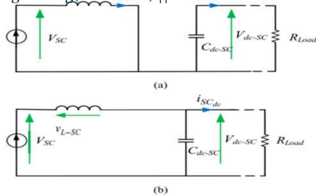
FIGURE5. Electrical scheme of a buck-
